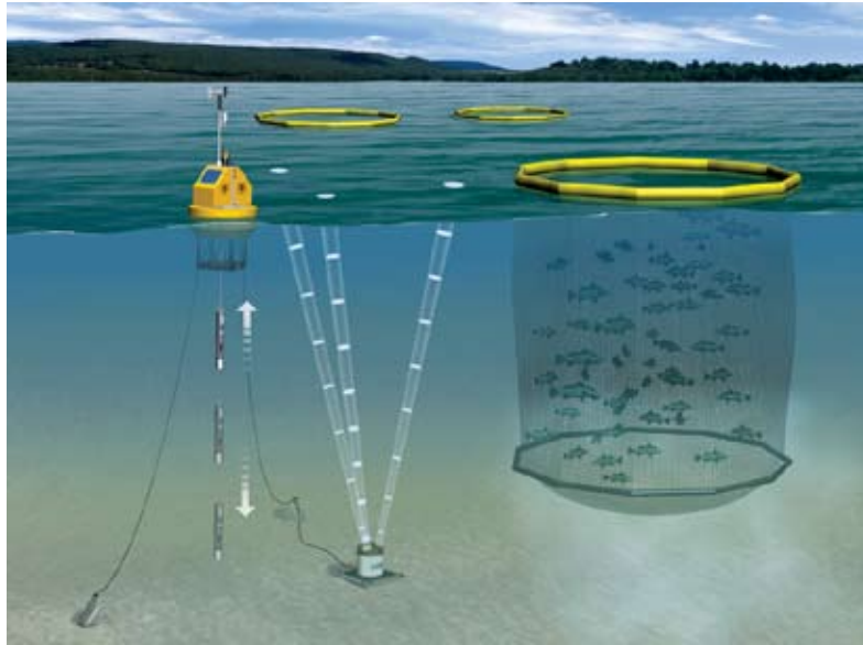
A complete YSI sea cage monitoring solution. A YSI buoy with a vertical profiling 6600 V2 along with a SonTek/YSI Argonaut provides continuous monitoring of water quality, current and wave data.
